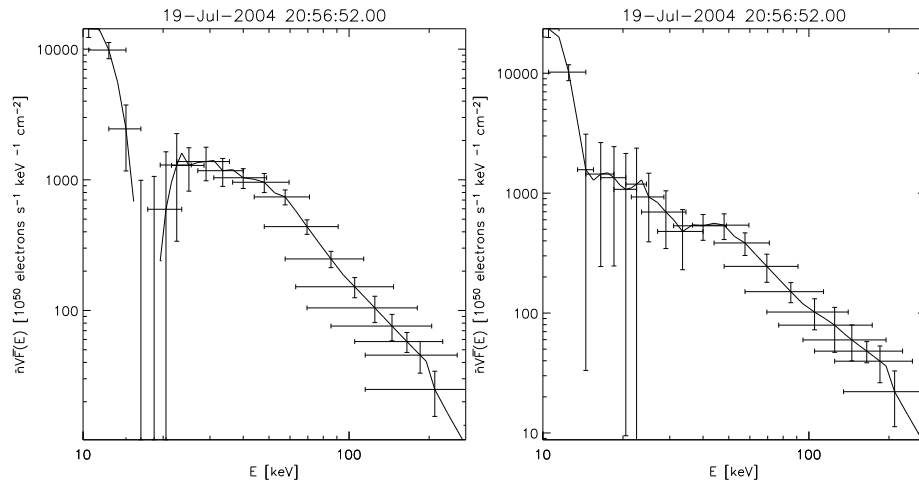
Fig. 7. \bar{F}(E) corresponding to the total (left) and primary (right) flare photon spectrum for an event close to the disc centre (19 Jul 2004). Vertical error bars correspond to 3\sigma uncertainties, horizontal lines show the FWHM of energy resolution determined from regularised inversion.
